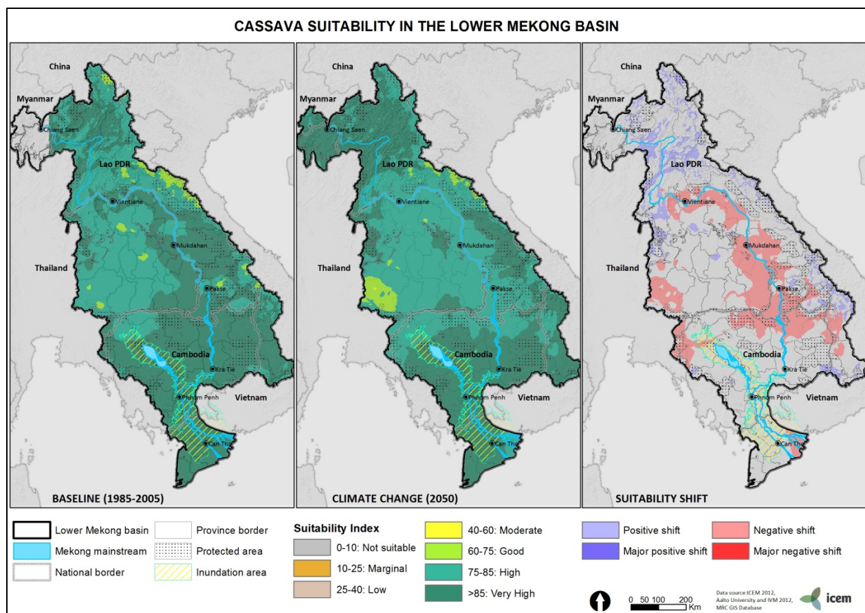
Figure 23: Baseline and 2050 land suitability of cassava in the Lower Mekong Basin
