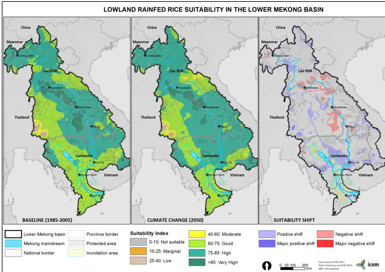
Figure 21: Baseline and 2050 land suitability for lowland rainfed rice (planted date in May, 150 days) in the Lower Mekong Basin
