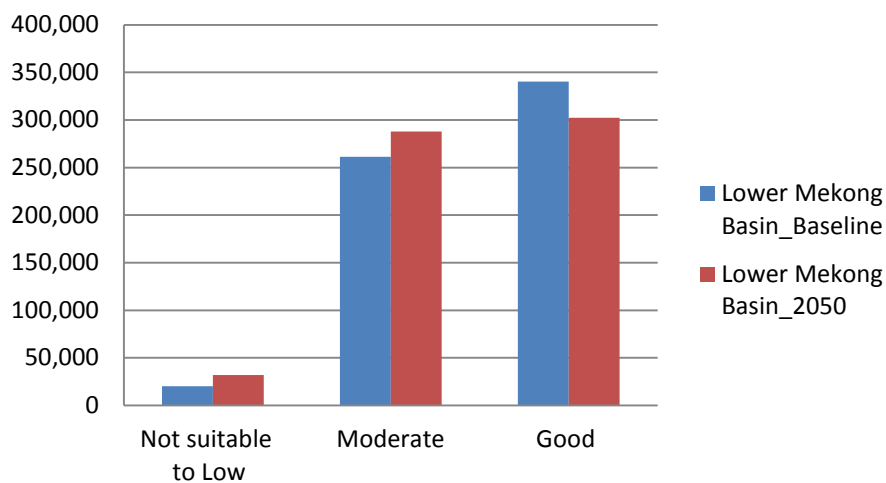
Figure 26: Change in climate suitability area from baseline to 2050 for the entire Lower Mekong Basin for maize cultivation (planting date in May)
